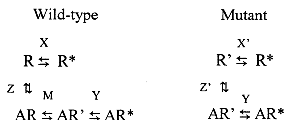
Scheme 3. Agonist induction mechanism with pre-active species.
